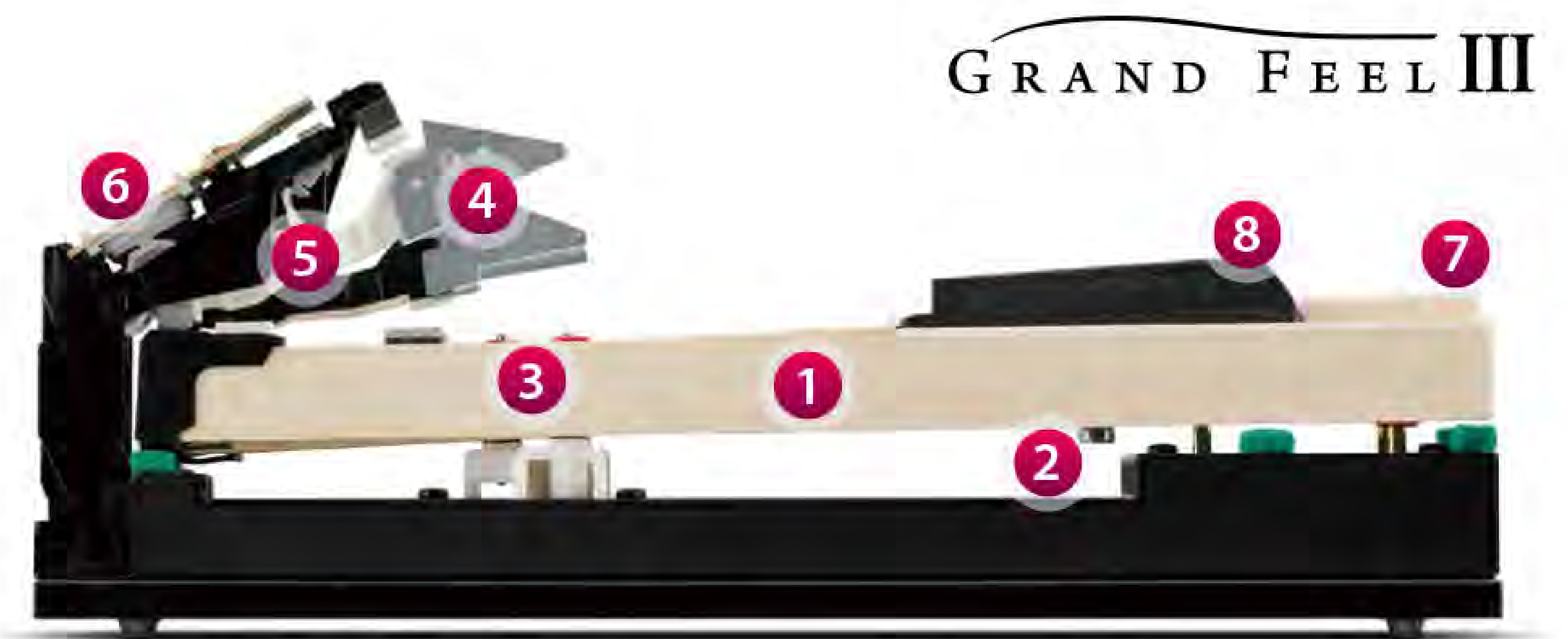
Grand Feel III action (CA79/CA99)
